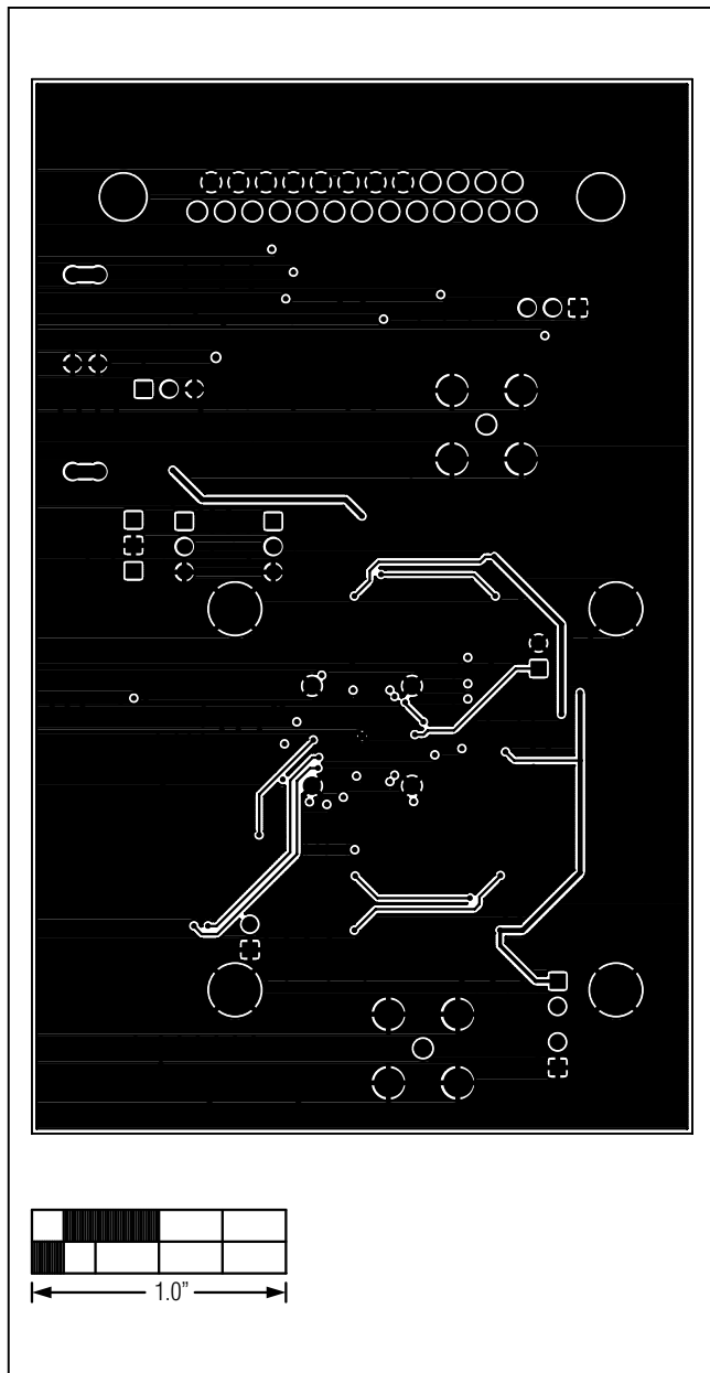
Figure 5. MAX2140 EV Kit PCB Layout—Layer 3
