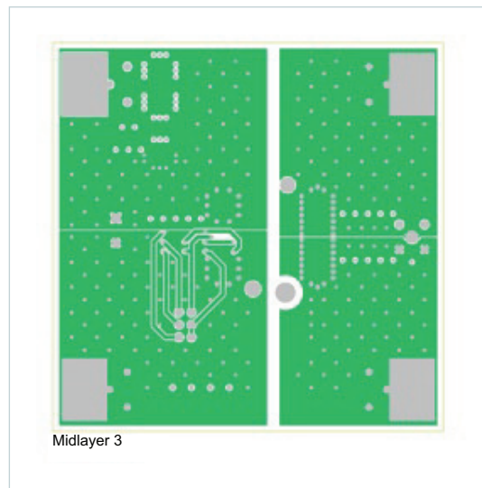
Figure 10. Midlayer 3 Artwork 2 Oz. Copper
