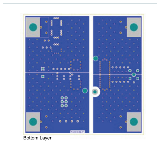
Figure 12. Bottom Layer Artwork 3 Oz. Copper
