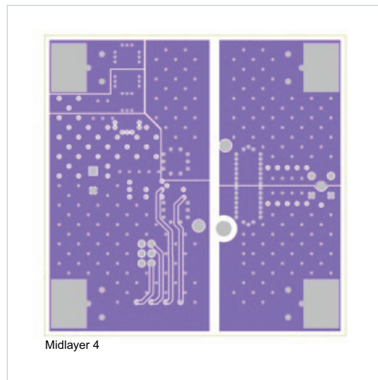
Figure 11. Midlayer 4 Artwork 2 Oz. Copper
