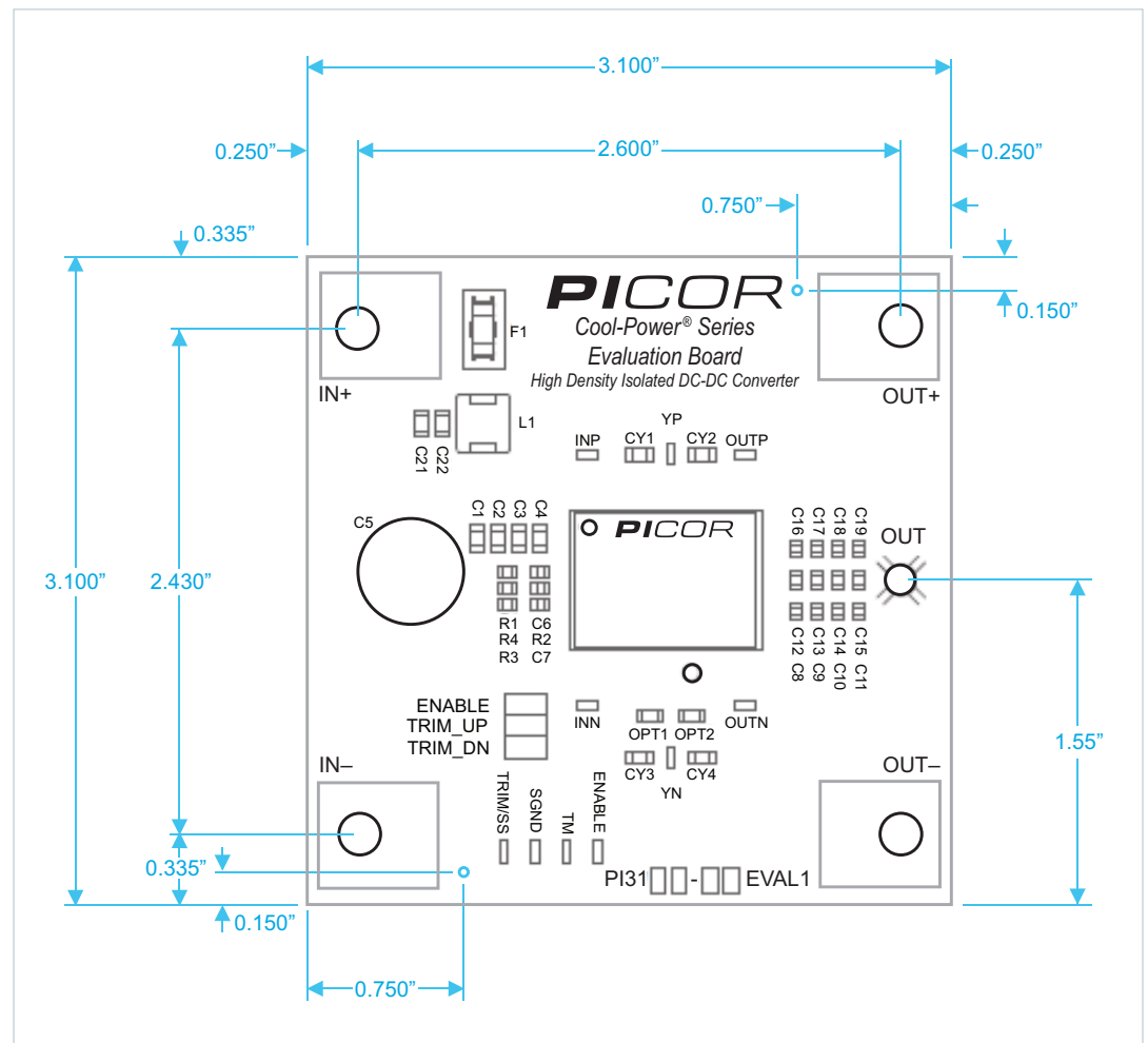
Figure 13. Mechanical Drawing
