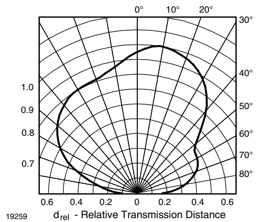
Fig. 13 - Vertical Directivity
