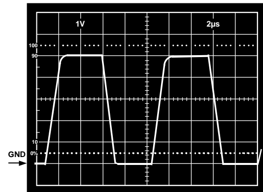
Figure 40. V_S = 5\text{ V} , 0\text{ V} ; Gain-of-2 Inverter Response to 2.5 V Step, Centered -1.25\text{ V} Below Ground, R_L = 10\text{ k}\Omega
