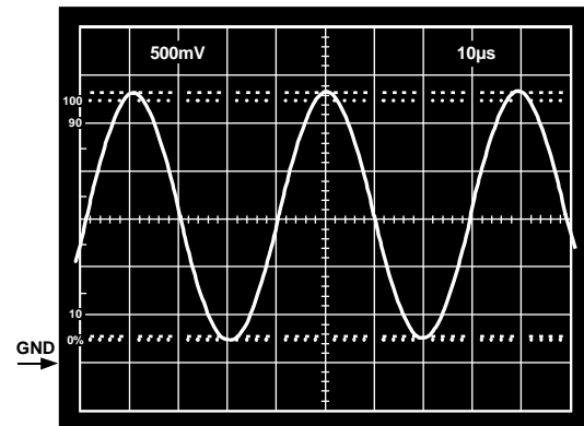
Figure 41. V_S = 3\text{ V} , 0\text{ V} ; Gain-of-2 Inverter, V_{IN} = 1.25\text{ V} , 25 kHz, Sine Wave Centered at -0.75\text{ V} , R_L = 600\ \Omega
