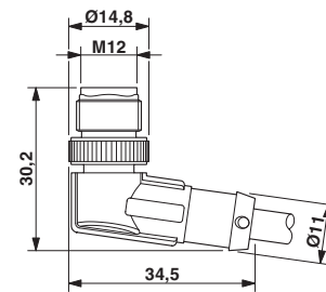
Dimensioned drawing
