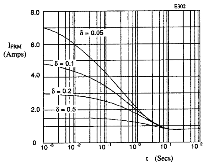
Fig 8. Maximum repetitive forward current as a function of pulse width at 100°C; R_{\theta JL} = 110\text{ }^{\circ}\text{C/W} ; V_{RWM} during 1 - \delta .
