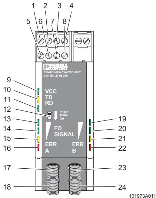
Figure 3 Function elements
