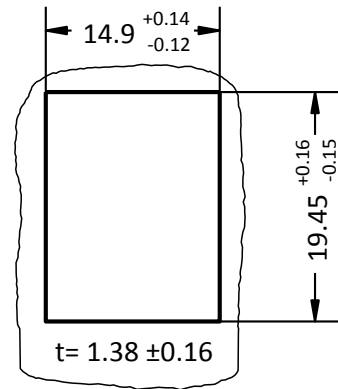
Figure 2. Suggested Keystone Cut-out
