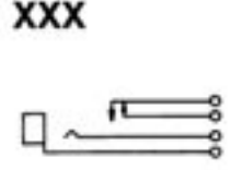
Single open circuit—“make” before “break”. (J11).
