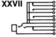
Tip closed; ring open circuits. Isolated switching—two “make” circuits and one “break” circuit. (J10-2A-1B).
