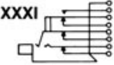
Tip closed; ring closed circuits. Isolated switching—“break” before “make” circuit.
