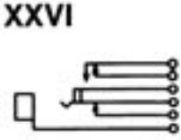
Single closed circuit. Isolated switching—“make” before “break” circuit. (J4-1D).
