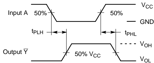
Figure 5. Switching Waveforms
