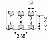
Underside View
