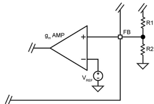
Figure 7. Voltage-Divider Configuration
