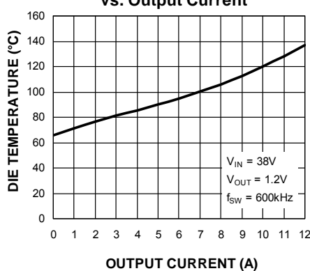
Die Temperature* ( V_{IN} = 38V ) vs. Output Current
