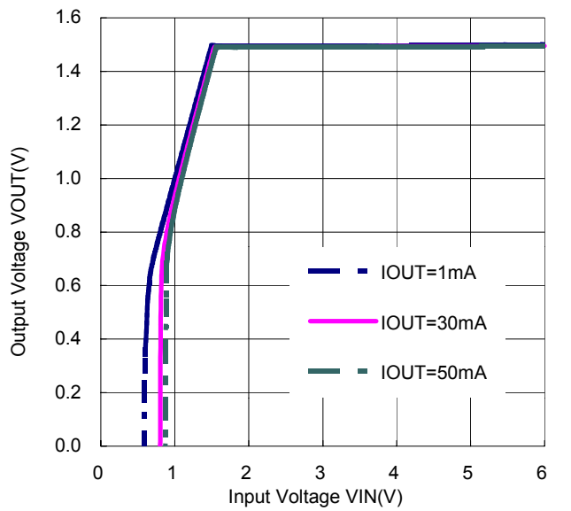
R1160N151X ECO=L
