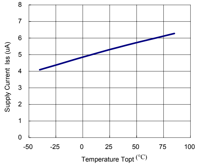
R1160N331X ECO=L
