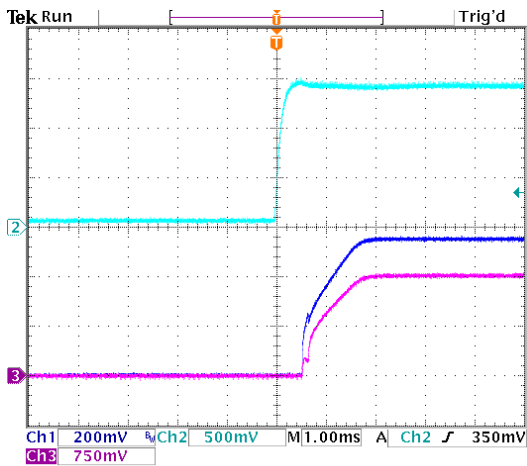
Figure 6. Typical Start-Up Using Remote On/Off ( V_o = 0.6Vdc , I_o=20A ). Ch1 - Vout, Ch2 - ON/OFF, Ch3 - Iout
