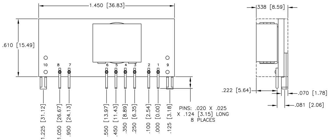
Figure 23. Mechanical Drawing
