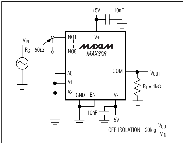
Figure 6. Off-Isolation
