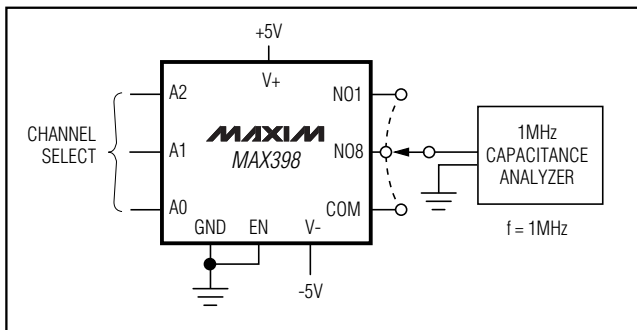
Figure 8. NO/COM Capacitance
