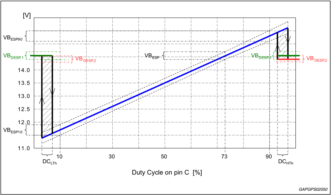
Figure 4. External regulation curve versus C duty cycle @ T_J = 30\text{ °C} and F duty cycle = 15%
