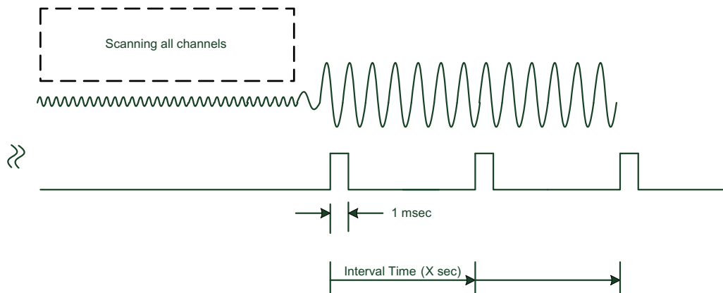
Figure 33. Energysense Signal Wakeup Logic
