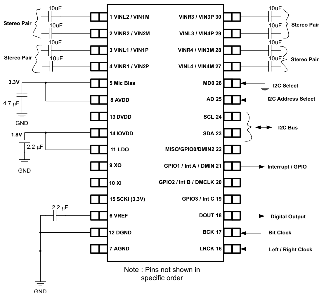
Figure 58. Simplified Schematic, PCM1863 I²C Controlled Subsystem
