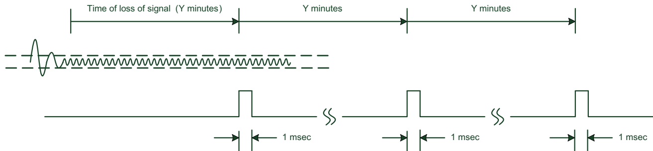
Figure 32. Interrupt Behavior for Signal Loss.
