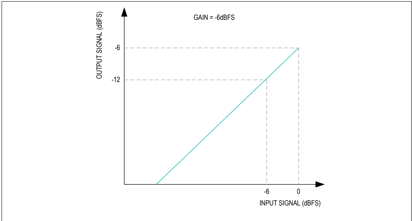
Figure 22. Gain Reduction Profile Example with -6dB Setting
