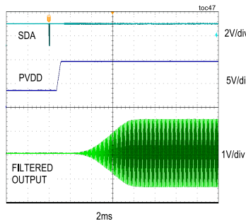
SYSTEM TURN-ON RESPONSE VOLUME RAMP ENABLED
