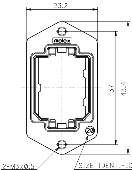
2-M3x0.5 SIZE IDENTIFICATION
