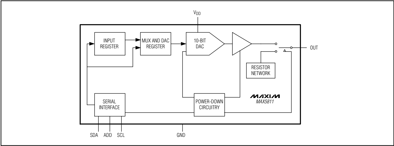
Functional Diagram
