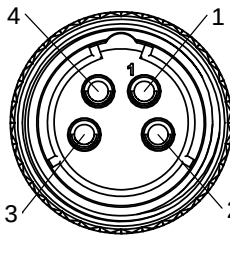
WIRE VIEW SF8382-4PG-5XX
