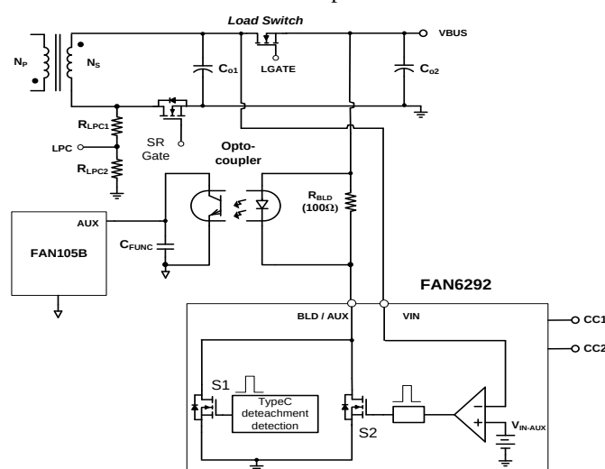
Figure 14 BLD/AUX Function Diagram
