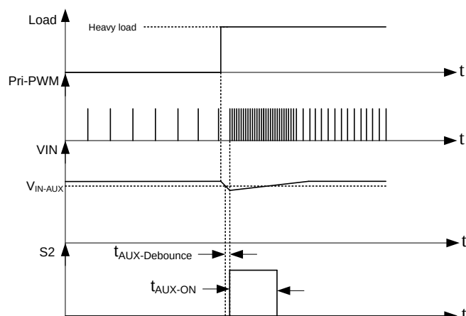
Figure 15 VIN-UV Protection
