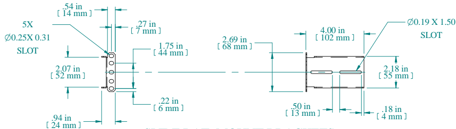
ASSEMBLED VIEW
