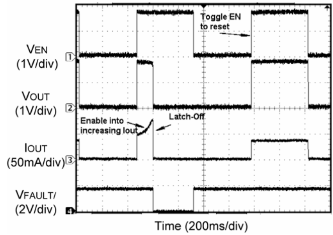
Overcurrent Lathch-Off and Recovery (-2 Version)
