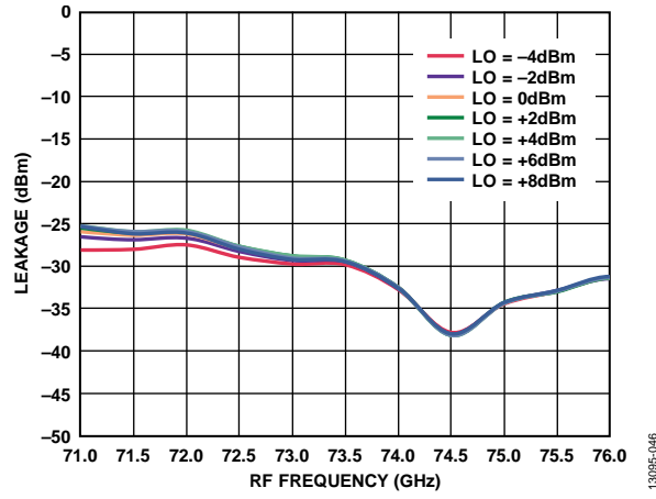
Figure 45. 6x LO Leakage at RFOUT vs. RF Frequency at Various LO Powers, IFIN = 5 dBm, IF = 2000 MHz, LSB
