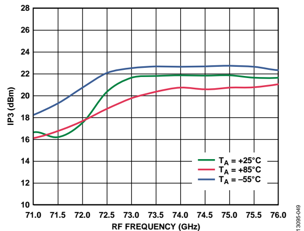
Figure 48. Input IP3 vs. RF Frequency at Various Temperatures, I_{FIN} = 5 dBm, LO = 2 dBm, IF = 500 MHz, USB
