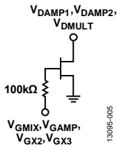
Figure 5. VGAMP, VGMIX, VDMULT, VDAMP1, VDAMP2, VGX2, VGX3 Interface
