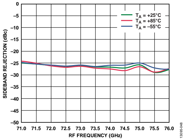
Figure 47. Sideband Rejection vs. RF Frequency at Various Temperatures, I_{FIN} = -8 dBm, LO = 2 dBm, IF = 500 MHz, USB
