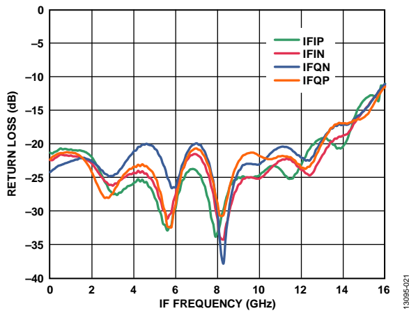
Figure 21. IF Port Return Loss vs. IF Frequency, LO = 2 dBm at LO = 12 GHz
