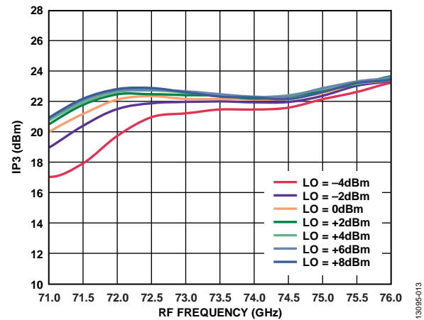
Figure 13. Input IP3 vs. RF Frequency at Various LO Powers, IF_{IN} = 5 \text{ dBm} , IF = 1000 \text{ MHz} , LSB
