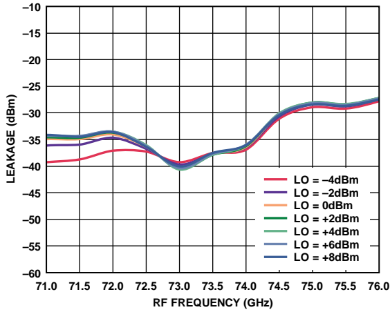
Figure 34. 6x LO Leakage at RFOUT vs. RF Frequency at Various LO Powers, I_{FIN} = 5 \text{ dBm} , IF = 500 \text{ MHz} , LSB
