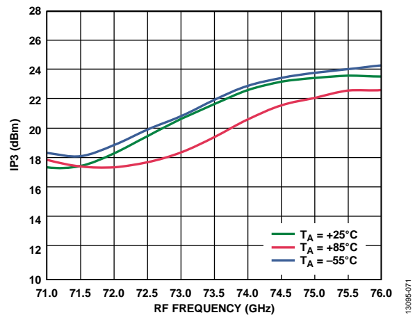
Figure 70. Input IP3 vs. RF Frequency at Various Temperatures, I_{FIN} = 5 dBm, LO = 2 dBm, IF = 2000 MHz, USB
