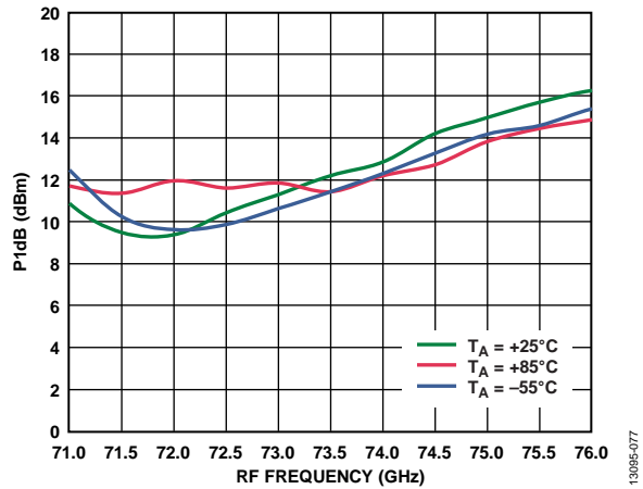
Figure 76. Input P1dB vs. RF Frequency at Various Temperatures, LO = 2 dBm, IF = 2000 MHz, USB
