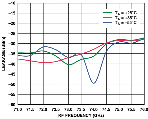
Figure 31. 6x LO Leakage at RFOUT vs. RF Frequency at Various Temperatures, I_{FIN} = 5 \text{ dBm} , LO = 2 \text{ dBm} , IF = 500 \text{ MHz} , LSB
