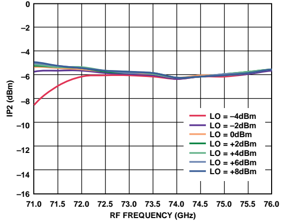
Figure 33. Input IP2 vs. RF Frequency at Various LO Powers, IFIN = 5 dBm, IF = 500 MHz, LSB
