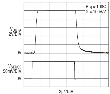
Amplifier Step Response ( V_{\text{SENSE}} = 0\text{mV} to 100mV)
