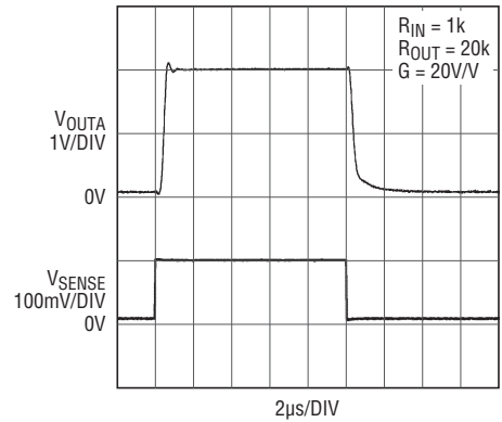
Amplifier Step Response ( V_{\text{SENSE}} = 10\text{mV} to 100mV)
