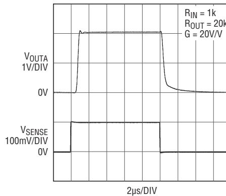
Amplifier Step Response ( V_{\text{SENSE}} = 0\text{mV} to 100mV)
