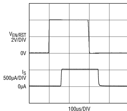
Enable/Disable Response
