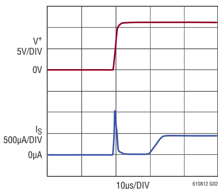
Start-Up Supply Current
