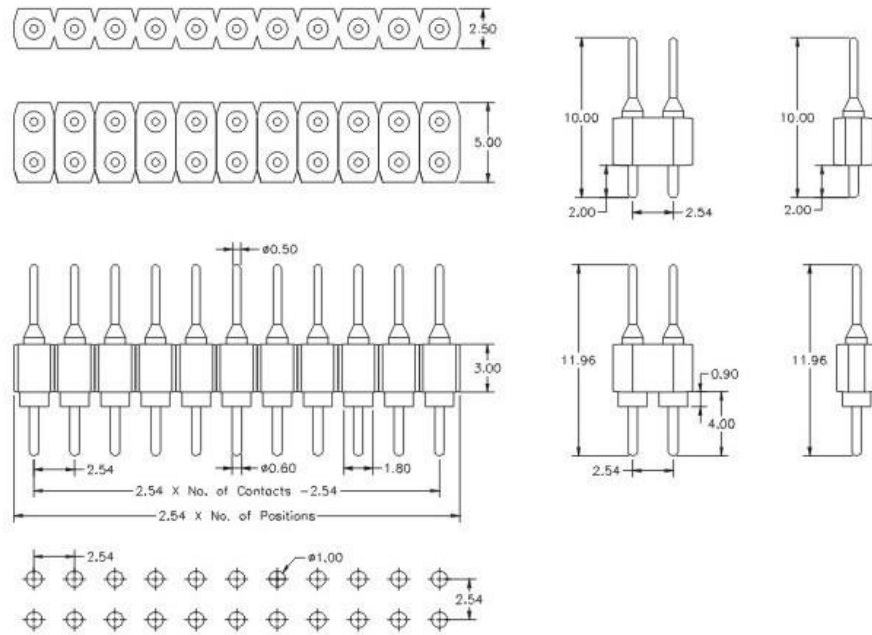
PCB LAYOUT
