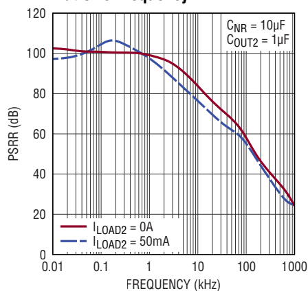
5V V_{OUT2} Power Supply Rejection Ratio vs Frequency
