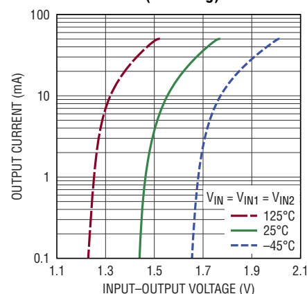
5V Minimum V_{IN} to V_{OUT2} Differential (Sourcing)
