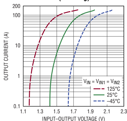
5V Minimum V_{IN} to V_{OUT1} Differential (Sourcing)
