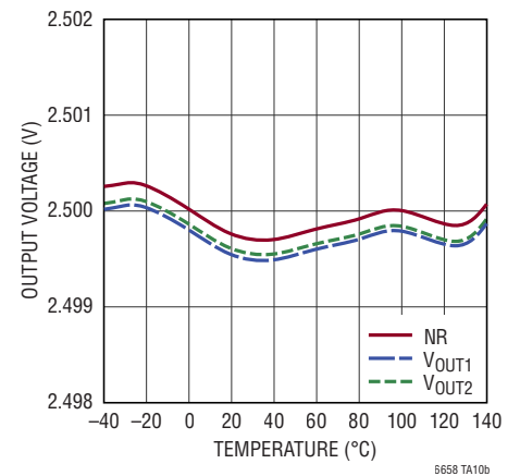
Precision Low Drift Application Drift = 1.5ppm/°C; -40°C to 125°C
