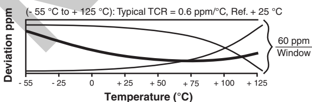
FIGURE 3 - TYPICAL CURVES WITHIN THE 60 ppm WINDOW, VHP100 TCR FOR MIL RANGE
