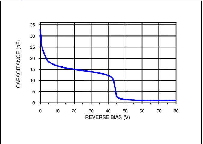
Fig.4 : APD CAPACITANCE vs BIAS VOLTAGE
