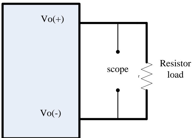
Figure 9: Output voltage noise and ripple measurement test setup
