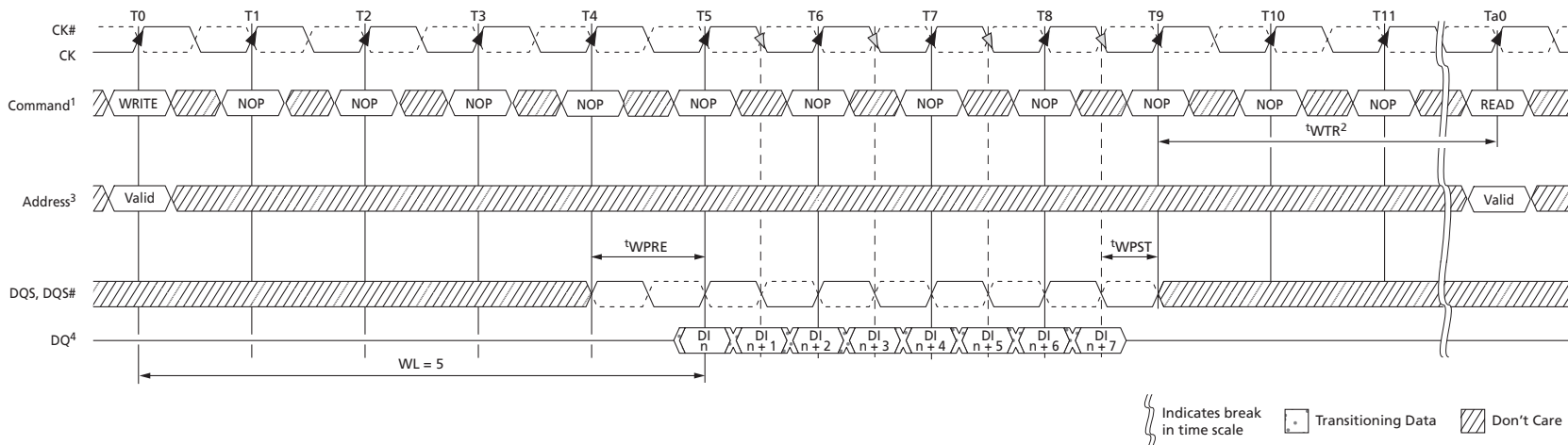
Figure 90: WRITE (BL8) to READ (BL8)
