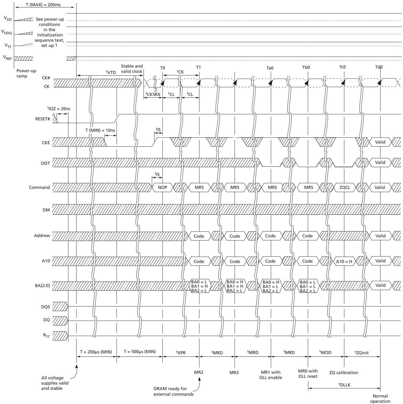
Figure 50: Initialization Sequence
