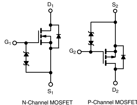
N-Channel MOSFET
