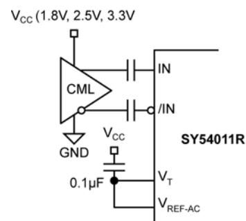
Figure 4c. CML Interface (AC-Coupled)
