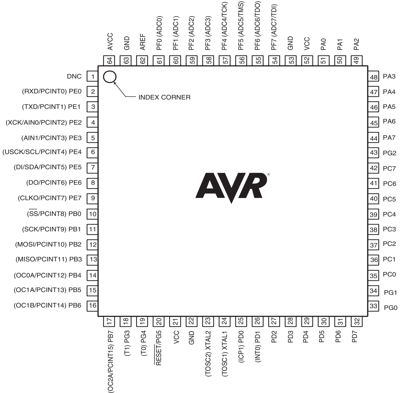
Figure 1-1. 64A (TQFP)and 64M1 (QFN/MLF) pinout Atmel ATmega165A/ATmega165PA/ATmega325A/ATmega325PA/ATmega645A/ATmega645P.
