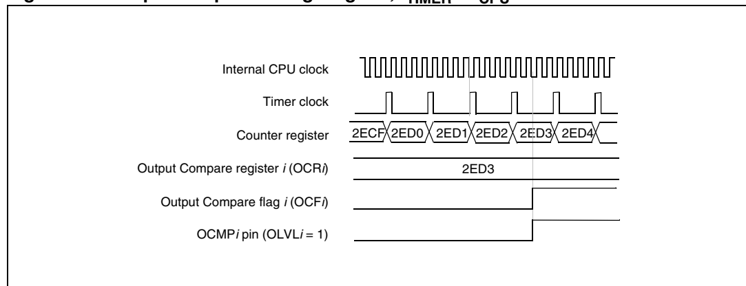
Figure 43. Output compare timing diagram, f_{\text{TIMERB}} = f_{\text{CPU}}/4
