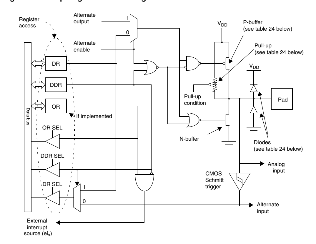
Figure 28. I/O port general block diagram
