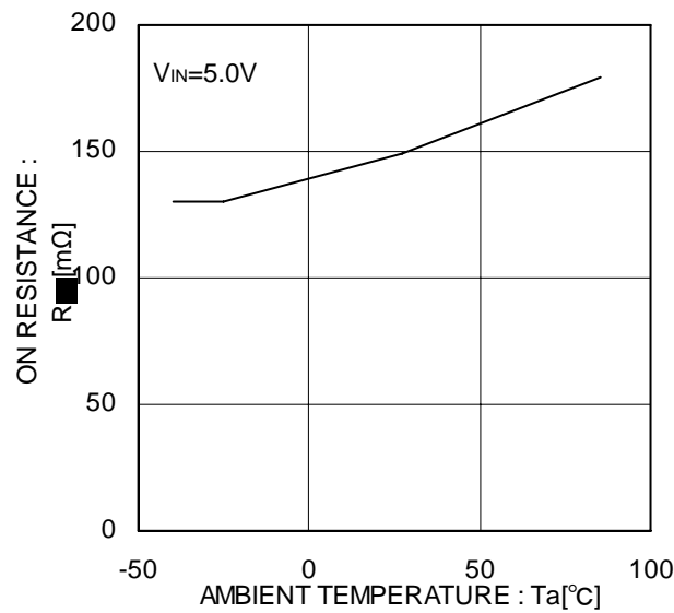
Figure 10. ON resistance
