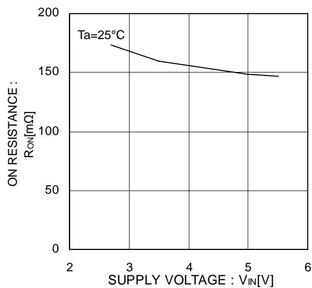
Figure 9. ON resistance
