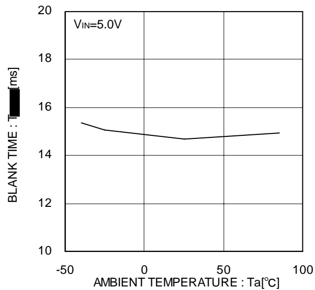
Figure 26. Blanking time
