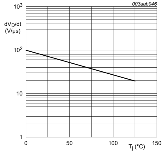
Fig. 14. Rate of rise of off-state voltage as a function of junction temperature; typical values
