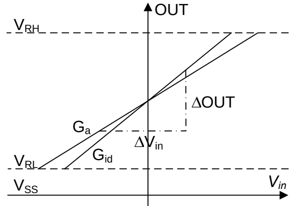
Figure 11: Gain definition
