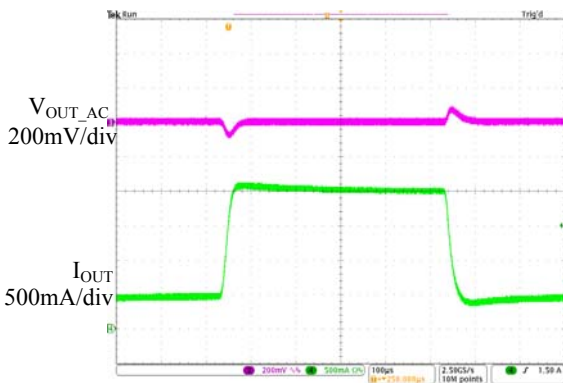
Time 100μs/div
