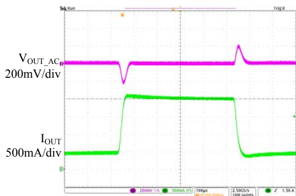
Time 100μs/div
