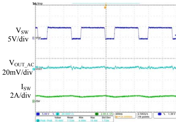
Time 400ns/div
