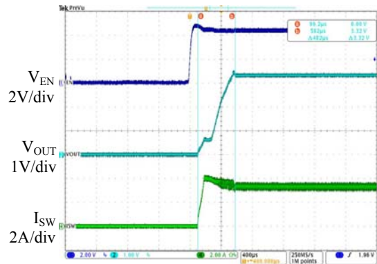
Time 400µs/div
