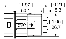
Short Depth - For Solder Termination to PCB
