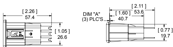
Flush Mount - For Crimp Termination to Wire
