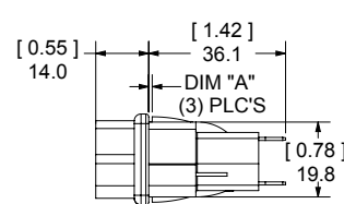
Short Depth - For Solder Termination to PCB
